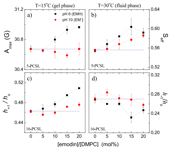
Fig. 5. Effect of emodin on the membrane structure of 10 mM DMPC, at pH 6.0 (black squares) and pH 10.0 (red circles), probed by 5-PCSL ( A_{\max} and S_{\text{eff}} , for the gel and fluid phases, respectively) and 16-PCSL ( h_{+1}/h_0 and h_{-1}/h_0 , for the gel and fluid phases, respectively). (a) and (c) gel phase at 15 °C, and (b) and (d) fluid phase at 30 °C. The dashed lines are only guide for the eyes and represent the values obtained without emodin. (For interpretation of the references to colour in this figure legend, the reader is referred to the web version of this article.)
