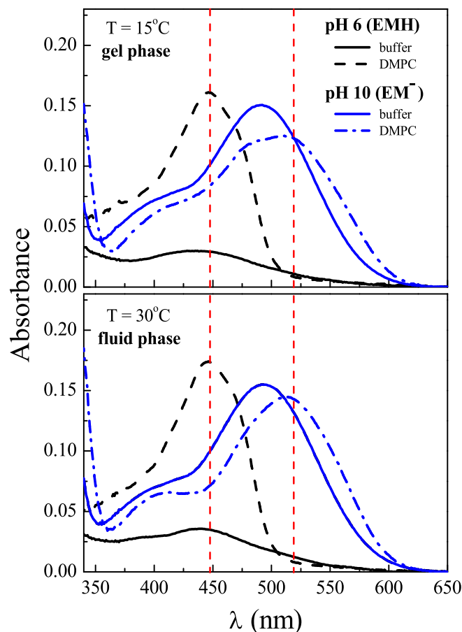
Fig. 3. Optical absorption spectra of 0.025 mM of emodin, neutral at pH 6.0 (EMH, black lines) and anionic at pH 10.0 ( EM^- , blue lines), in buffer solution (solid lines) and in DMPC (1 mM) dispersion (dash lines and dash dot lines), at T = 15 °C (gel phase) and T = 30 °C (fluid phase). Emodin/DMPC = 2 mol%. Dashed vertical red lines are just guides for the eyes, drawn at wavelength values 446 and 519 nm. (For interpretation of the references to colour in this figure legend, the reader is referred to the web version of this article.)
